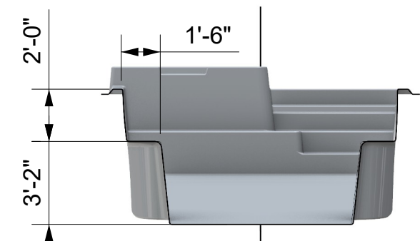
(B) LEDGE DETAIL
