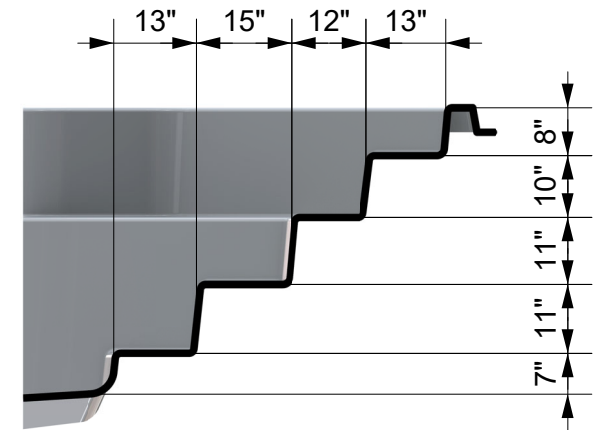
A STEP DETAIL
