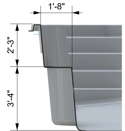
B LEDGE DETAIL
