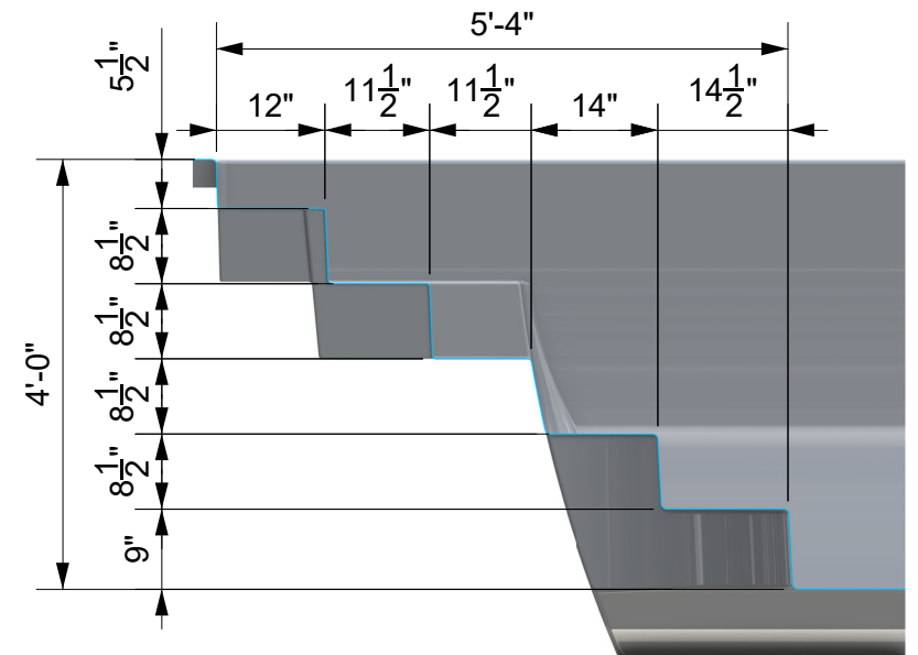
A STEP DETAIL
